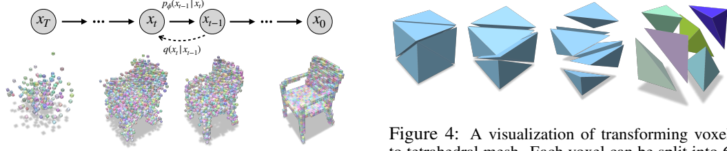
Figure 3: Generating voxelized shapes with DDPM.
