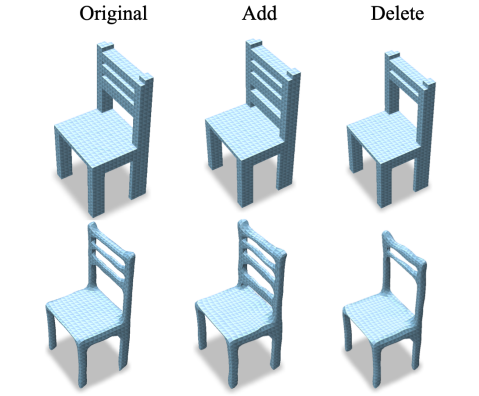
Figure 10: An application in shape editing where the user edits the coarse voxel shape and the final shape is updated accordingly
