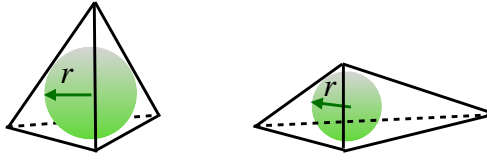
Figure 16: Green sphere: inscribed sphere of the tetrahedron with radius r . The left tetrahedron is a regular one, while the tetrahedron is a distorted one. A highly distorted tetrahedron will hurt the down-stream performance of the generated volumetric mesh.
